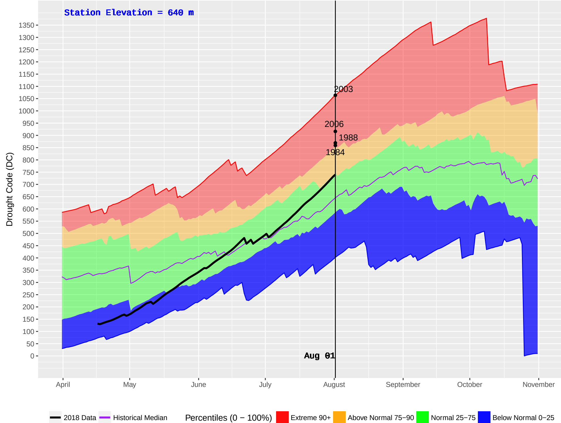
MERRITT HUB (294) : Historical (1978–2016) and Current (2018) Daily Drought Code (DC)
