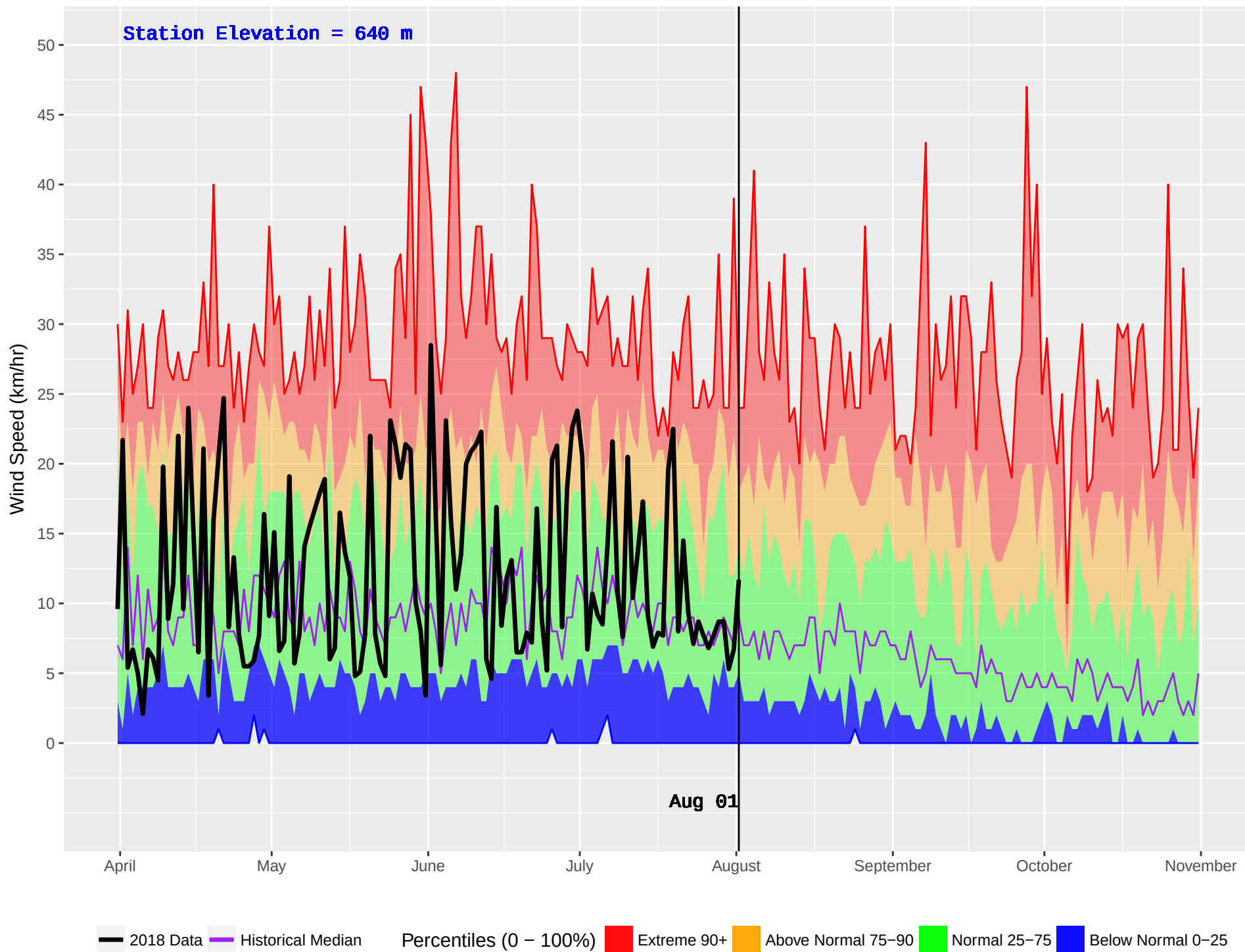
MERRITT HUB (294) : Historical (1978–2016) and Current (2018) Daily Wind Speed
