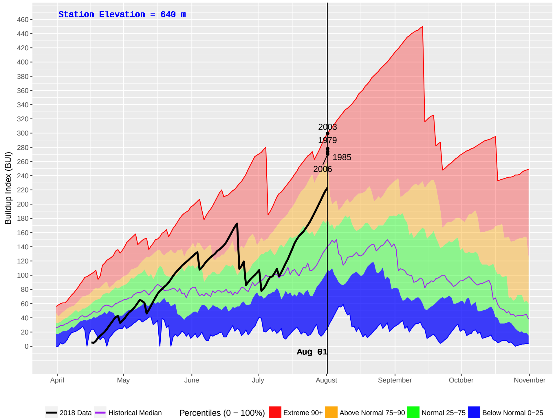
MERRITT HUB (294) : Historical (1978–2016) and Current (2018) Daily Buildup Index (BUI)
