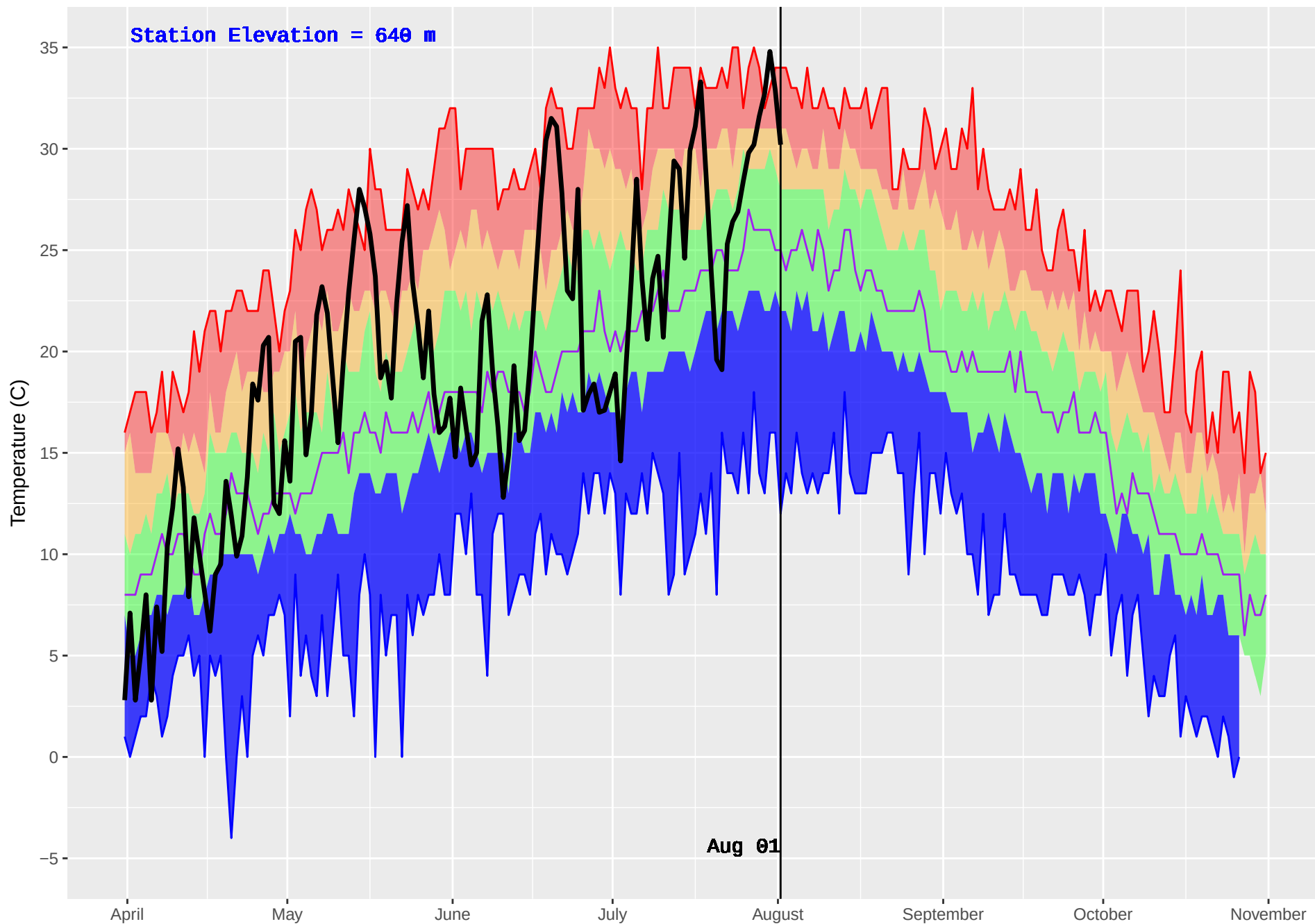
MERRITT HUB (294) : Historical (1978–2016) and Current (2018) Daily Temperature
