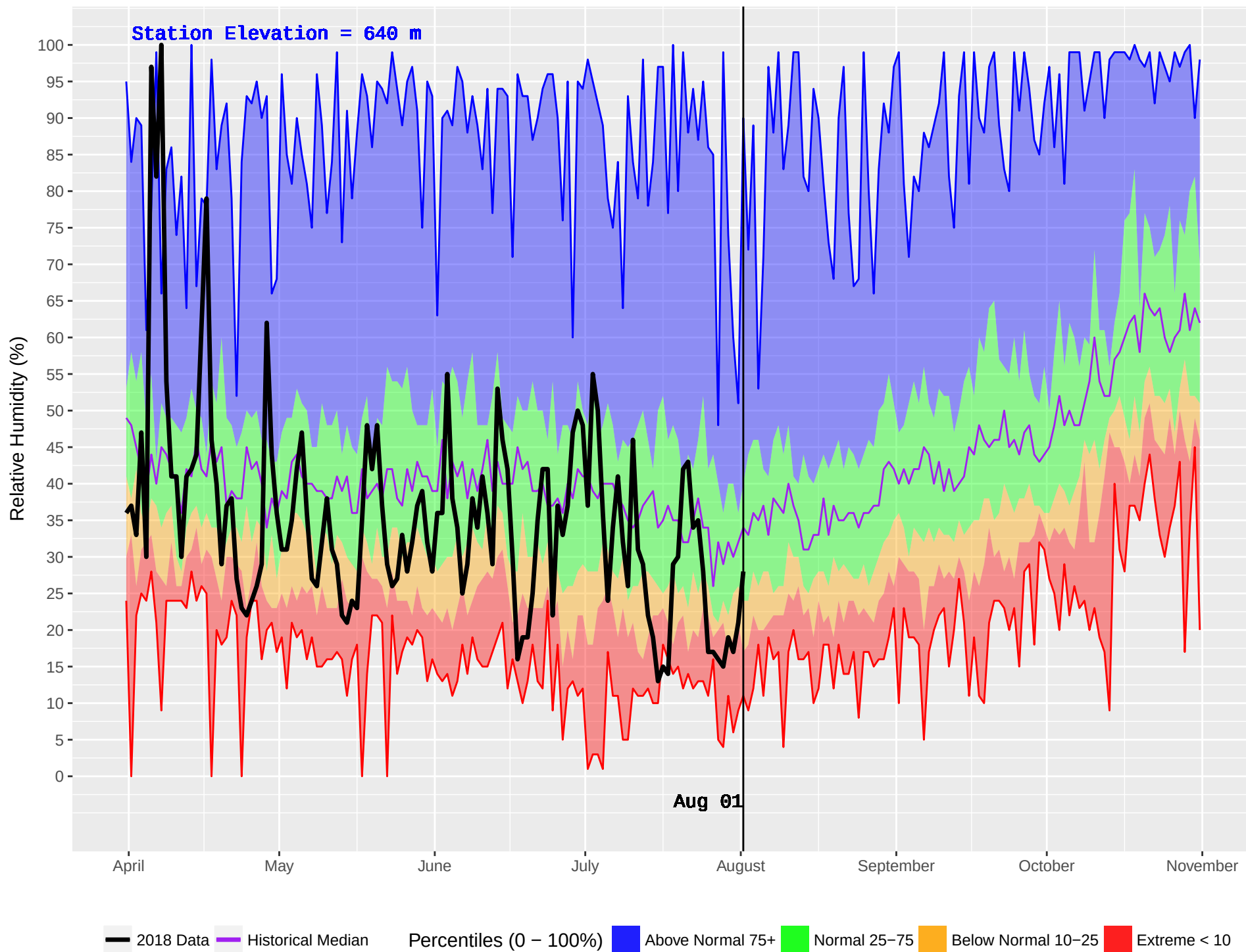
MERRITT HUB (294) : Historical (1978–2016) and Current (2018) Daily Relative Humidity
