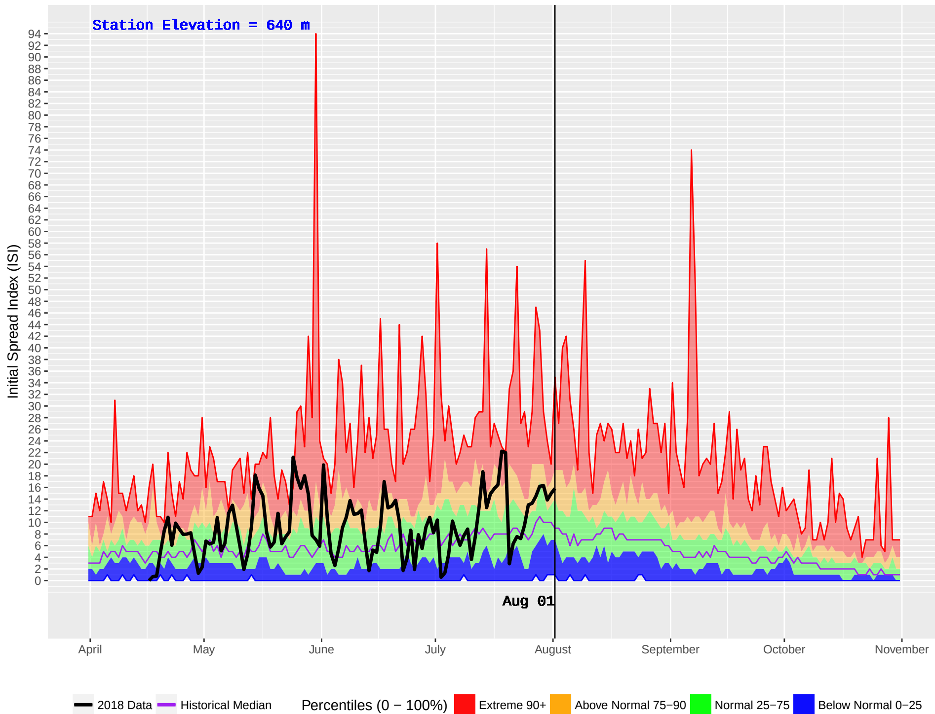
MERRITT HUB (294) : Historical (1978–2016) and Current (2018) Daily Initial Spread Index (ISI)
